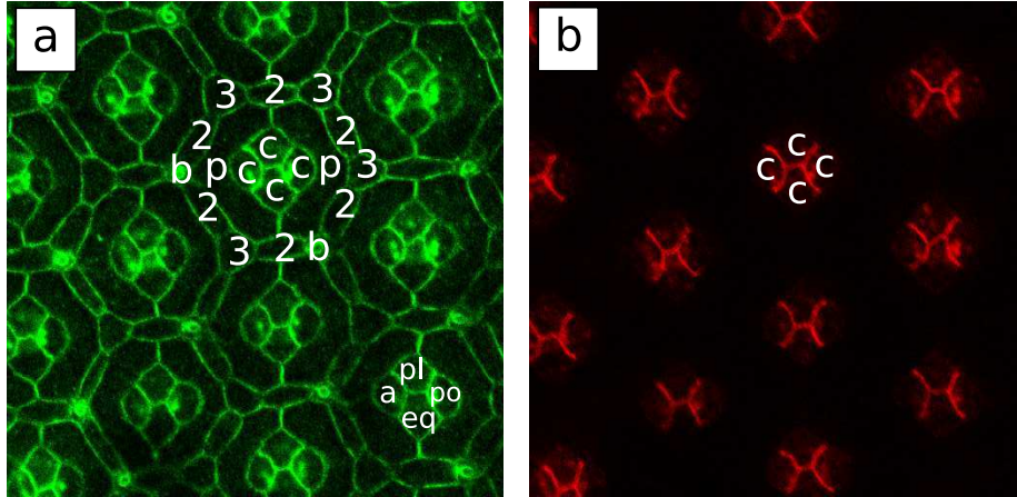
Fig. 7. Confocal microscopy images of the Drosophila retina. The pictures measure 100 \mu\text{m} \times 100 \mu\text{m} . (a) b-Catenin, a component of the adherens junction, is stained green. Nearly all catenin fluorescence between the cone cells is seen in a layer of 1.26 \mu\text{m} thick. One ommatidium consists of four cone cells (c) and two primary pigment cells (p), surrounded by six secondary (2) and three tertiary (3) pigment cells and three bristle cells (b). In this particular ommatidium, one bristle cell is replaced by a tertiary pigment cell. The cone cells can be subdivided into a polar (pl), equatorial (eq), anterior (a) and posterior (po) cone cell, according to their position. (b) N-cadherin fluorescence in the same plane of focus. N-cadherin is restricted to the cone-cone interfaces.
