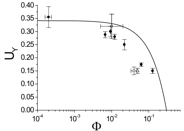
Fig. 11. Yield strain versus liquid fractions for the different setups of Figure 1: \circ , (a); \bullet , different experiments of (b); \square , (c); \Delta , (d). Trend of data (b) can be qualitatively compared to a quadratic law [30]: U_Y = C(\Phi_c - \Phi)^2 , with \Phi_c corresponding to the rigidity limit liquid fraction ( \approx 30\% for setup (b) [14]) and C an empirical constant equal to 1.1.
