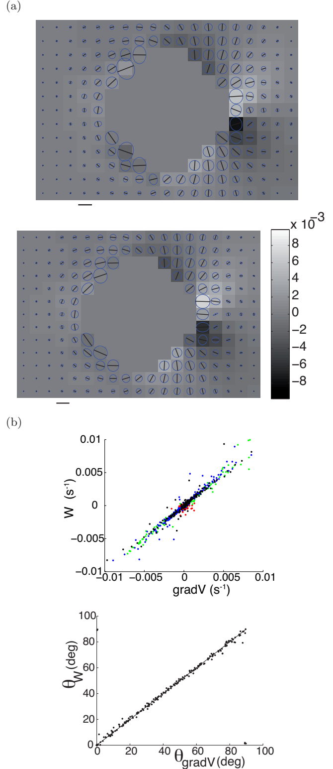
Fig. 3. Affine assumption: test of equation (8) on the foam of Figure 1b. (a) Comparison of maps of \mathbf{W} (top) and \nabla \mathbf{v} (bottom): ellipses, symmetric part; grey levels, antisymmetric part (bar: 5.6 \times 10^{-3} \text{ s}^{-1} ). (b) Quantitative comparison: top, (W_{XX} - W_{YY})/2 versus (\nabla v_{XX} - \nabla v_{YY})/2 , and the same for all other components (superimposed): XX + YY , XY - YX , XY + YX ; bottom, angle (in degrees) of ellipses plotted in (a). Each point comes from one RVE of the image.
