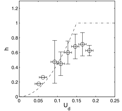
Fig. 13. Estimate of h . Symbols: measurements from Figure 1a of P_d/V_d \simeq h . We represented the average (circle) and standard deviation (vertical error bar) after binning data along the horizontal axis on equal interval sizes (horizontal error bar). Dash-dots: h(U_d) = \min((U_d/U_Y)^2, 1) , quadratic up to U_Y = 0.15 .
