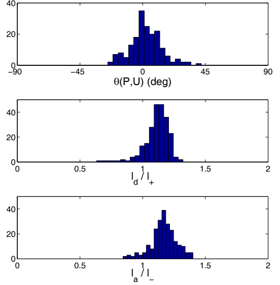
Fig. 7. Histograms of measurements in all regions of the foam (Fig. 1a). Top: angle between topological events and elongation. Middle: length of disappearing links compared to average length in elongation direction \ell_+ . Bottom: length of appearing links compared to average length in compressed direction \ell_- .
