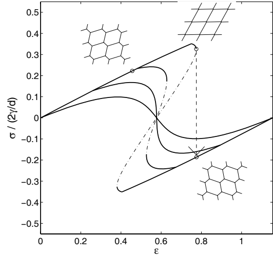
Fig. 6. Shear of a 2D ordered foam [22], different liquid fraction: 9.3% (close-packing, lowest amplitude curve), 5.5% (onset of a negative slope unstable branch), 3% and 1%. Decreasing liquid leads to increasing maximum stress. The topological rearrangement occurs when the stress versus strain curve becomes unstable (dot-dashed line) and induces an irreversible strain. Three 1% foams states are represented (circles on curve). The stress \sigma is here normalised using surface tension \gamma and bubble radius d .
