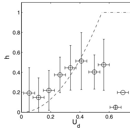
Fig. 15. Same figure as Figure 13, but for the dry foam of Figure 1b, U_Y = 0.45 .
