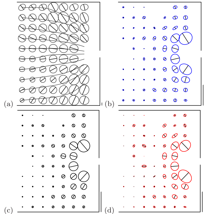
Fig. 16. Foam flowing through a constriction (Fig. 1c). Same caption as Figure 12, except that for \mathbf{U} bar = 0.1 , and for \mathbf{V} and \mathbf{P} bar = 0.25 \text{ s}^{-1} . See similar figures in the companion paper [14].
