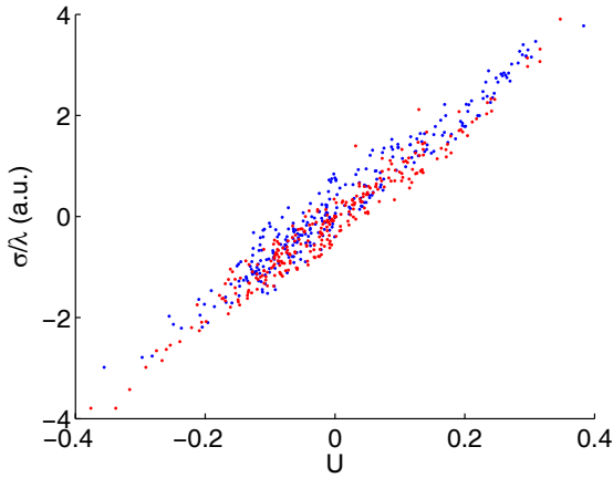
Fig. 4. XY components of the elastic stress \sigma (in arbitrary units) versus XY components of \mathbf{U} . Each point comes from one RVE of the image of Figure 1b. The slope of the cloud of points is the foam's 2D shear modulus; it is of order of the bubbles' line tension \lambda to diameter ratio. Data for the (XX - YY)/2 components are superimposed: they have the same slope.
