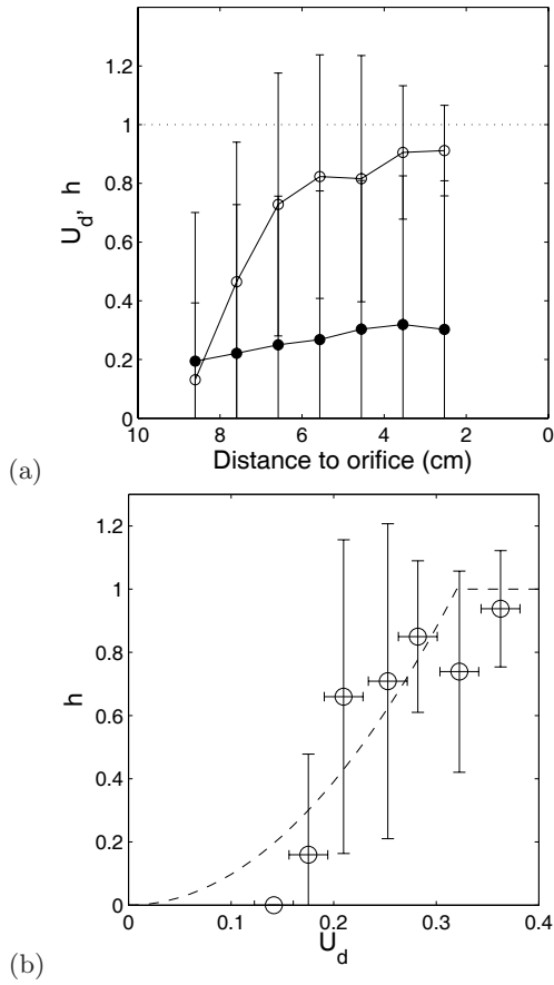
Fig. 17. Constriction: analysis of Figure 1c. (a) P_d/V_d (open circles) and U_d (closed circles) versus the distance to the constriction. (b) Plasticity fraction h estimated as h \simeq P_d/V_d versus strain U_d (data from (a)); same figure as Figures 13 and 15, here with U_Y = 0.32 .
