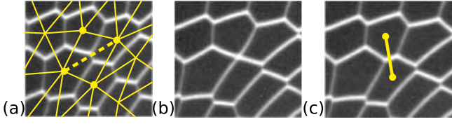
Fig. 2. Sequence of images of a T1 event in a measurement box: (a) shows the network of links \ell (thin lines) joining neighbour bubble centers superimposed on snapshots extracted from a dry foam [14], and the disappearing link ( \ell_d , dashes), (b) the intermediate stage, and (c) the appearing link ( \ell_a , thick line).
