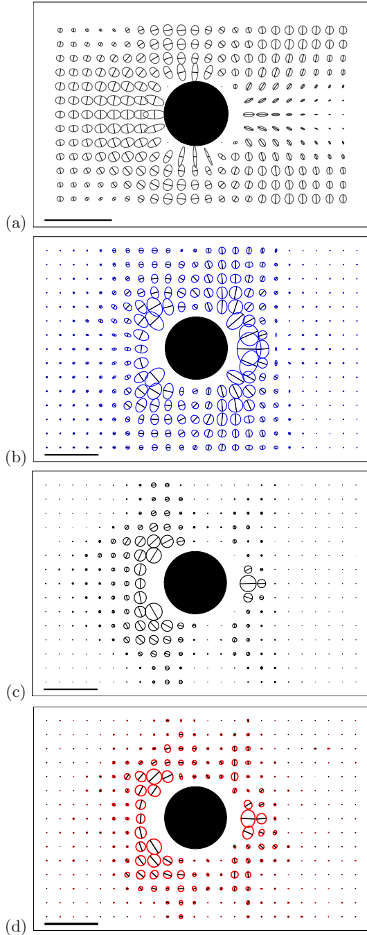
Fig. 12. Wet foam flowing around an obstacle (Fig. 1a). Measurements of \mathbf{U} (a) and \mathbf{V} (b) yield, through equation (14) with quadratic plasticity function h , the theoretical prediction of \mathbf{P} (c), in good agreement with its measurement (d). Scale: for \mathbf{U} , bar = 1 (no unit); for \mathbf{V} and \mathbf{P} : bar = 1 \text{ s}^{-1} .
