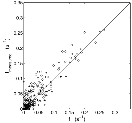
Fig. 8. Frequency of rearrangements: observed versus predicted. Each point corresponds to a RVE of the foam, that is, one ellipse of Figure 12. Observations: frequency f_{\text{measured}} of rearrangements (per link and second) measured in Figure 1a. Predictions: f from equation (18), setting the yield function to h = \min((U/U_Y)^2, 1) and the yield U_Y = 0.15 , while \varepsilon_0 = 1.2 (Eq. (20)). Solid line: diagonal f_{\text{measured}} = f .
