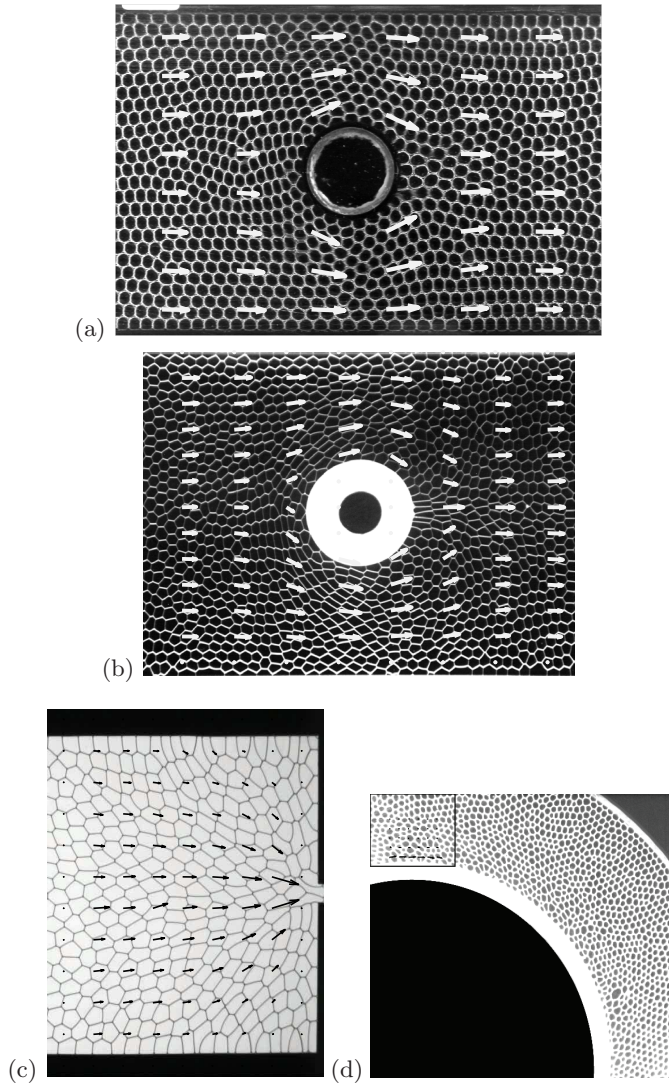
Fig. 1. Experimental 2D flows of a foam: top view, here flow from left to right. (a) Wet foam (between glass and water) flowing around an obstacle, picture from B. Dollet [15,16]; field of view 15\text{ cm} \times 10\text{ cm} . (b) Dry foam (between parallel glass plates) flowing around an obstacle, picture from C. Raufaste [14]; field of view 13.3\text{ cm} \times 10\text{ cm} . (c) Moderately dry foam (between parallel plexiglass plates) flowing through a narrow hole, picture from M. Asipauskas [17]; field of view 7.5\text{ cm} \times 10\text{ cm} . (d) Wet foam (between parallel glass plates) sheared between two concentric wheels with tooth-shaped boundaries to prevent slipping; the rotating inner wheel is visible at the bottom, the fixed outer wheel is visible at the top [18]. Arrows indicate the measured velocity field; field of view 12.5\text{ cm} \times 11.5\text{ cm} . Liquid fractions are approximately estimated as: (a) 4 \cdot 10^{-2} [19], (b) 2 \cdot 10^{-4} [20], (c) 10^{-2} [17], (d) 5 \cdot 10^{-2} [18].
