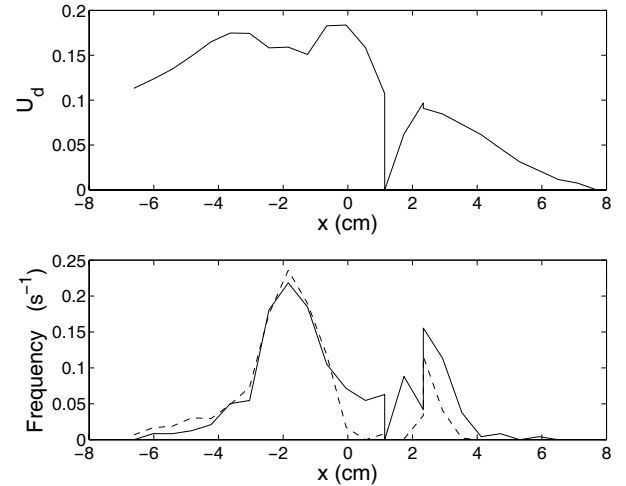
Fig. 10. Measurements along the streamline shown in Figure 9 bottom. Top: loading and unloading of elasticity, U_d . Bottom: T1 frequency along streamline, as in Figure 8; solid line: experimental f_{\text{measured}} ; dashed line: predicted f .
