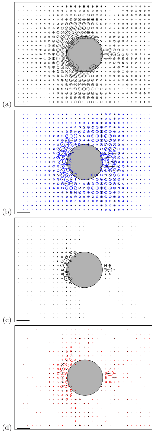
Fig. 14. Dry foam flowing around an obstacle (Fig. 1b). Same caption as Figure 12, except that for \mathbf{V} and \mathbf{P} bar = 0.063 \text{ s}^{-1} . See similar figures in the companion paper [14].
