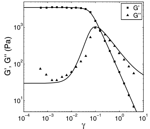
Fig. 19. Storage and loss moduli versus strain amplitude for a monodisperse emulsion. Symbols: experimental G' (squares) and G'' (triangles) in a close-packed emulsion (Fig. 1 of Ref. [31]). Lines: model calculated with the complete set of equations (21–25). The method is the same as in reference [9]; the correspondence between scalars and matrices is obtained by replacing (\sigma, U, \dot{\epsilon}) with (\sigma_{xy}, 2U_{xy}, 2V_{xy}) . The factors 2 come from the tensorial generalization (Eq. (25)) of the scalar equation (Eq. (4)); this is why the yield strain is half of that used for the scalar case (Fig. 9 of Ref. [9]). The parameters are directly obtained from the experimental data: shear modulus G = 1.7 \cdot 10^3 Pa, yield strain U_Y = 0.0223 , and viscosity \eta = 30 Pa.s. The yield function used here is h = (U/U_Y)^2 .
