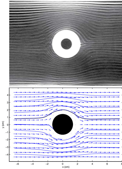
Fig. 9. Foam flow. Top: superimposed images evidence the streamlines (here from Fig. 1b). Bottom: measured velocity field and streamlines. The thicker solid line highlights the streamline analysed in Figure 10.
